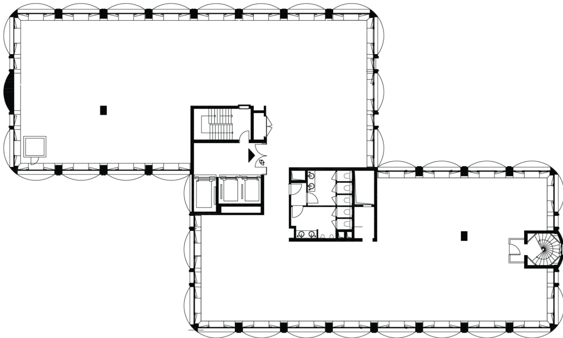
STANDARD PLAN FLOORS 1 TO 6
